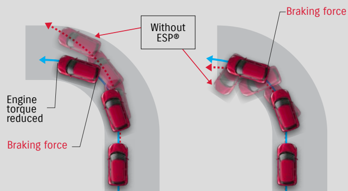
Front wheel slip
